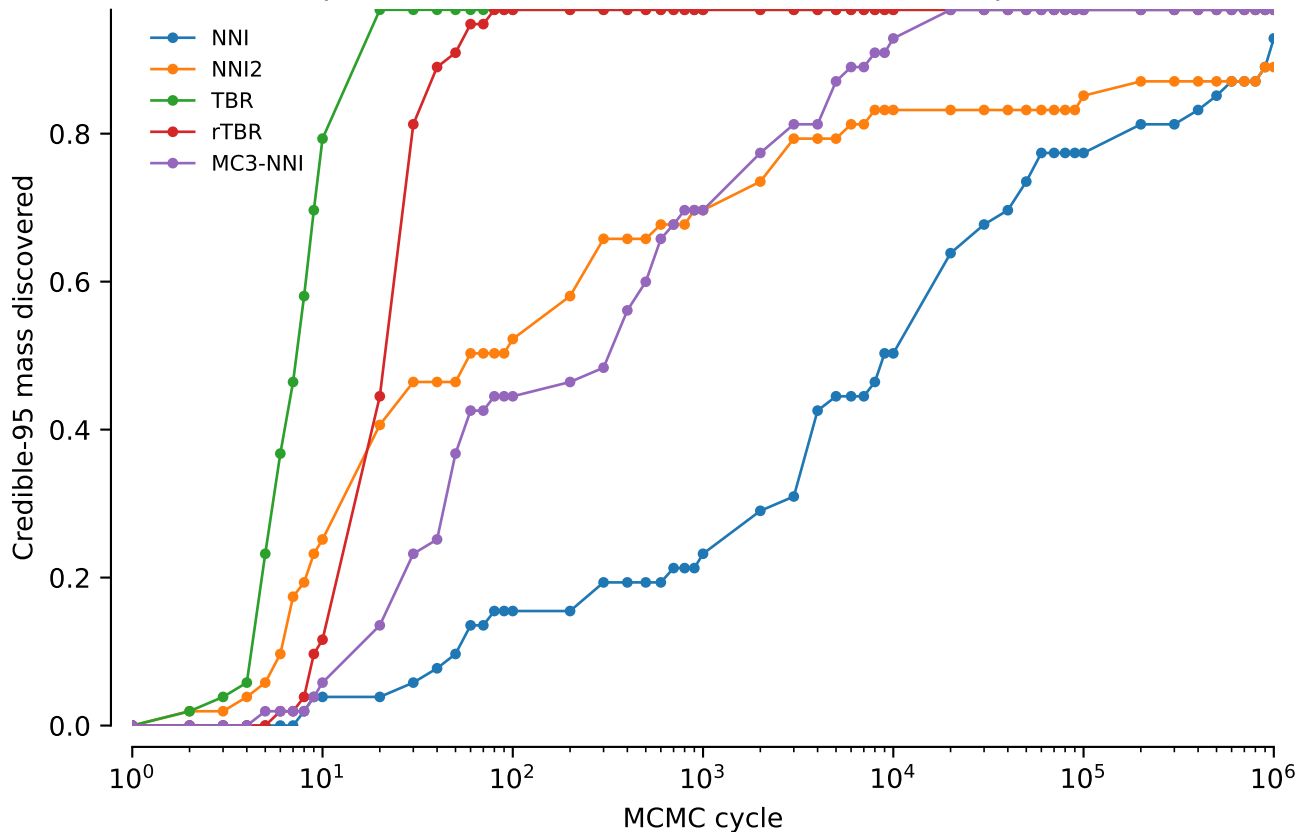
vert.atpase8.tw0: Credible-95 mass discovered: power = 0.3
