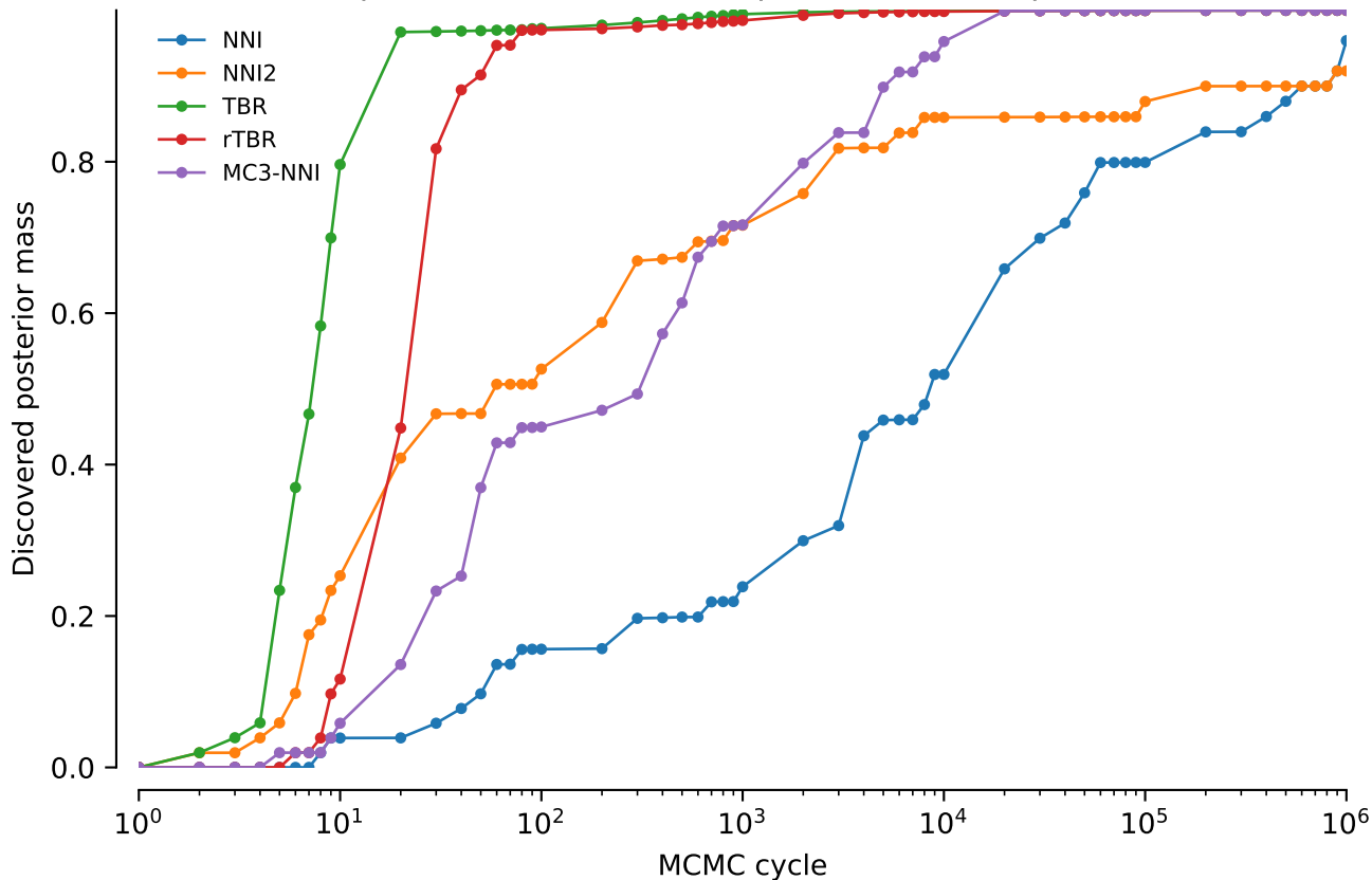
vert.atpase8.tw0: Discovered posterior mass: power = 0.3
