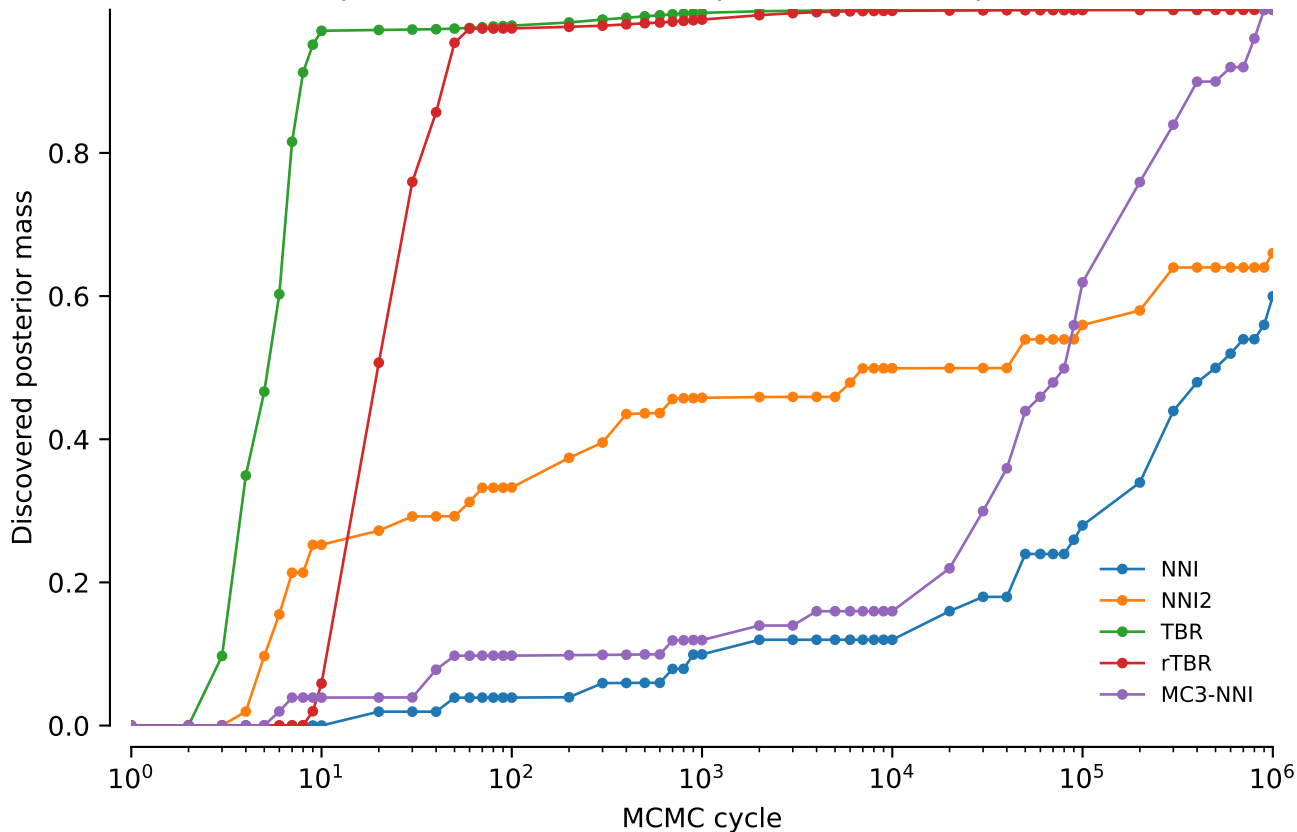
vert.atpase8.tw0: Discovered posterior mass: power = 0.4
