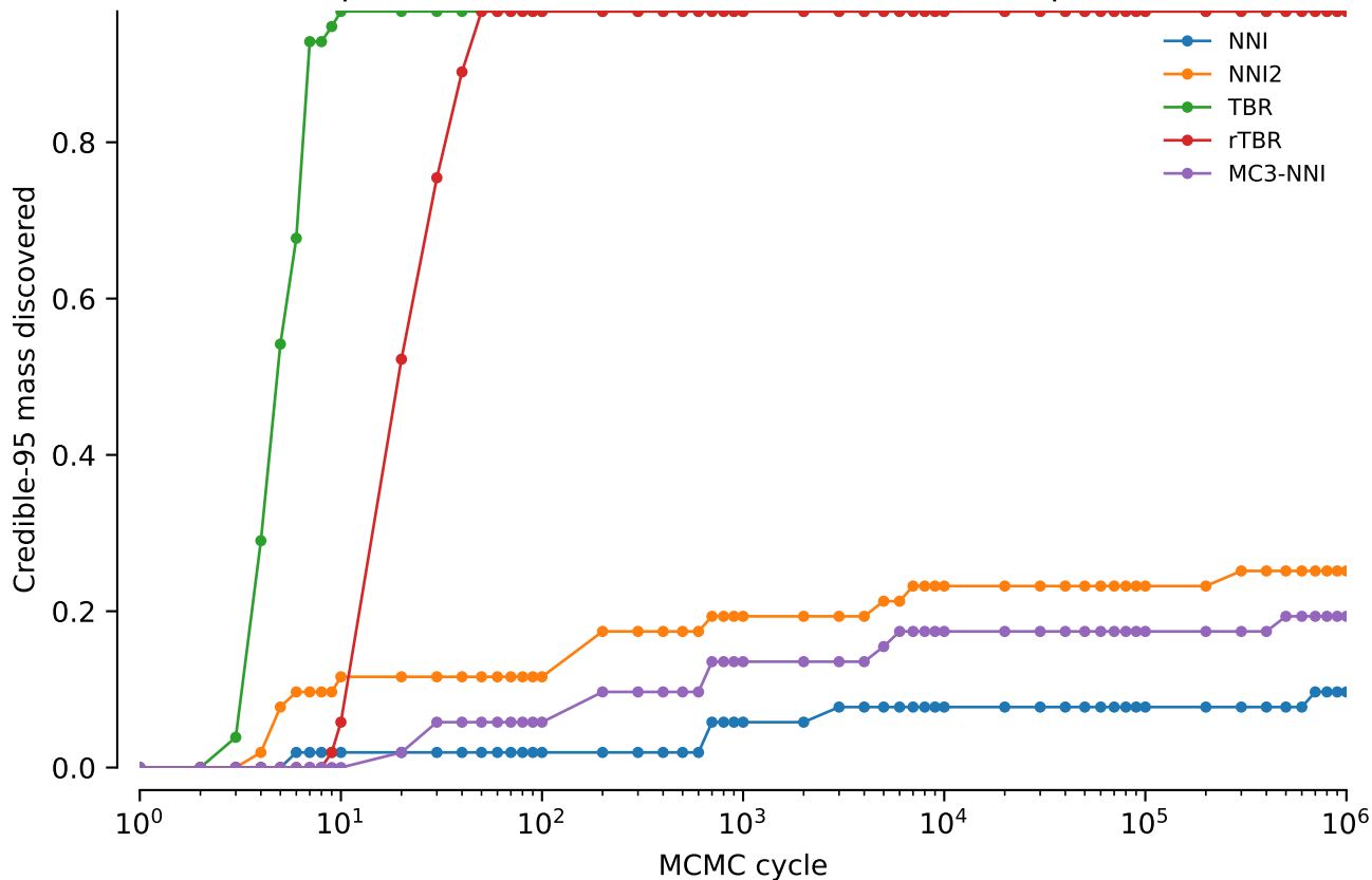
vert.atpase8.tw0: Credible-95 mass discovered: power = 0.5
