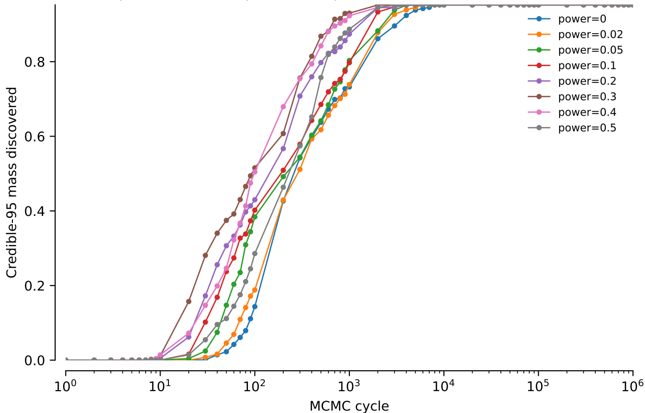
vert.atpase8.tw5: NNI power comparison: Credible-95 mass discovered
