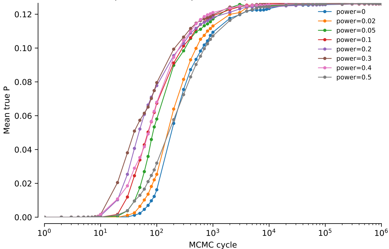
vert.atpase8.tw5: NNI power comparison: Mean true P
