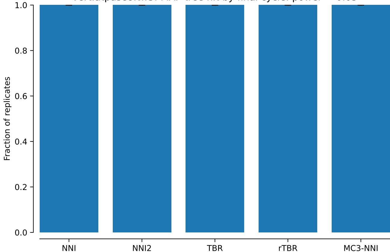
vert.atpase8.tw5: MAP tree hit by final cycle: power = 0.05
