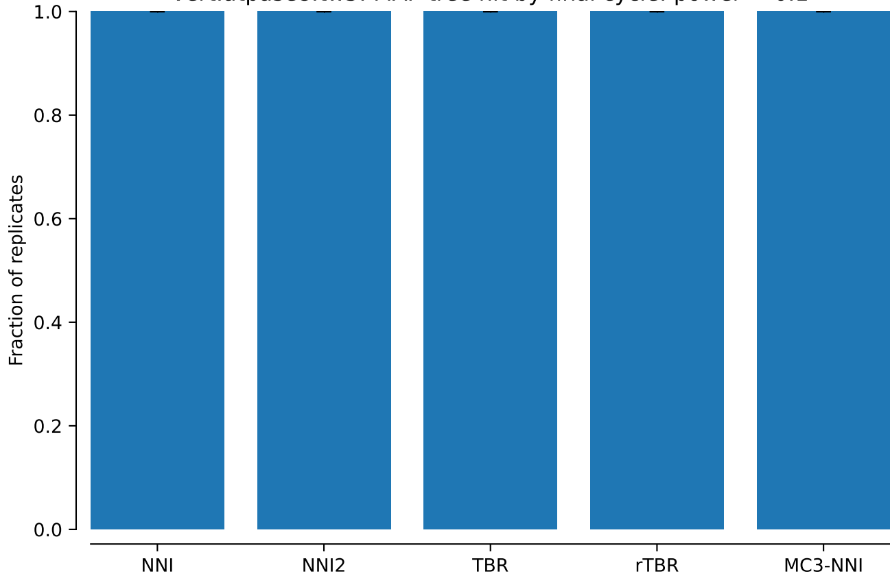
vert.atpase8.tw5: MAP tree hit by final cycle: power = 0.1
