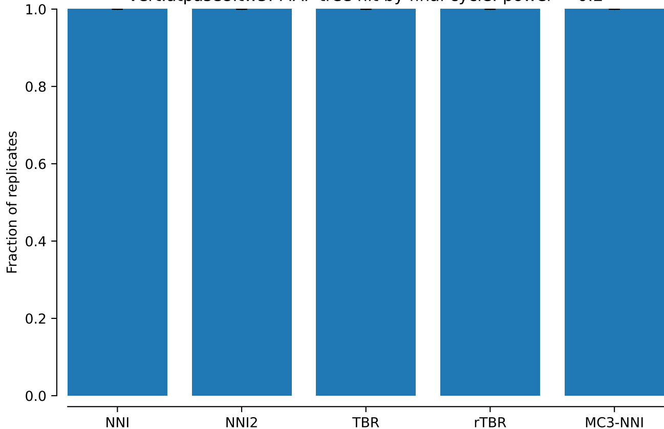
vert.atpase8.tw5: MAP tree hit by final cycle: power = 0.2
