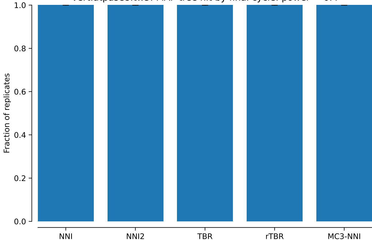
vert.atpase8.tw5: MAP tree hit by final cycle: power = 0.4
