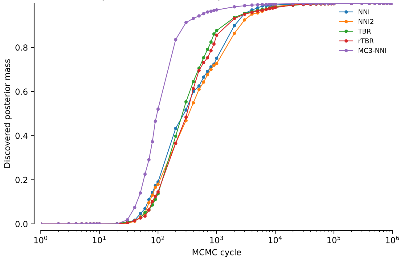
vert.atpase8.tw5: Discovered posterior mass: power = 0.02
