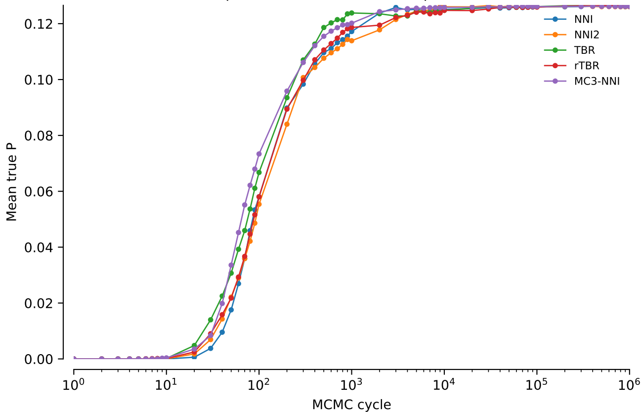
vert.atpase8.tw5: Mean true P: power = 0.05
