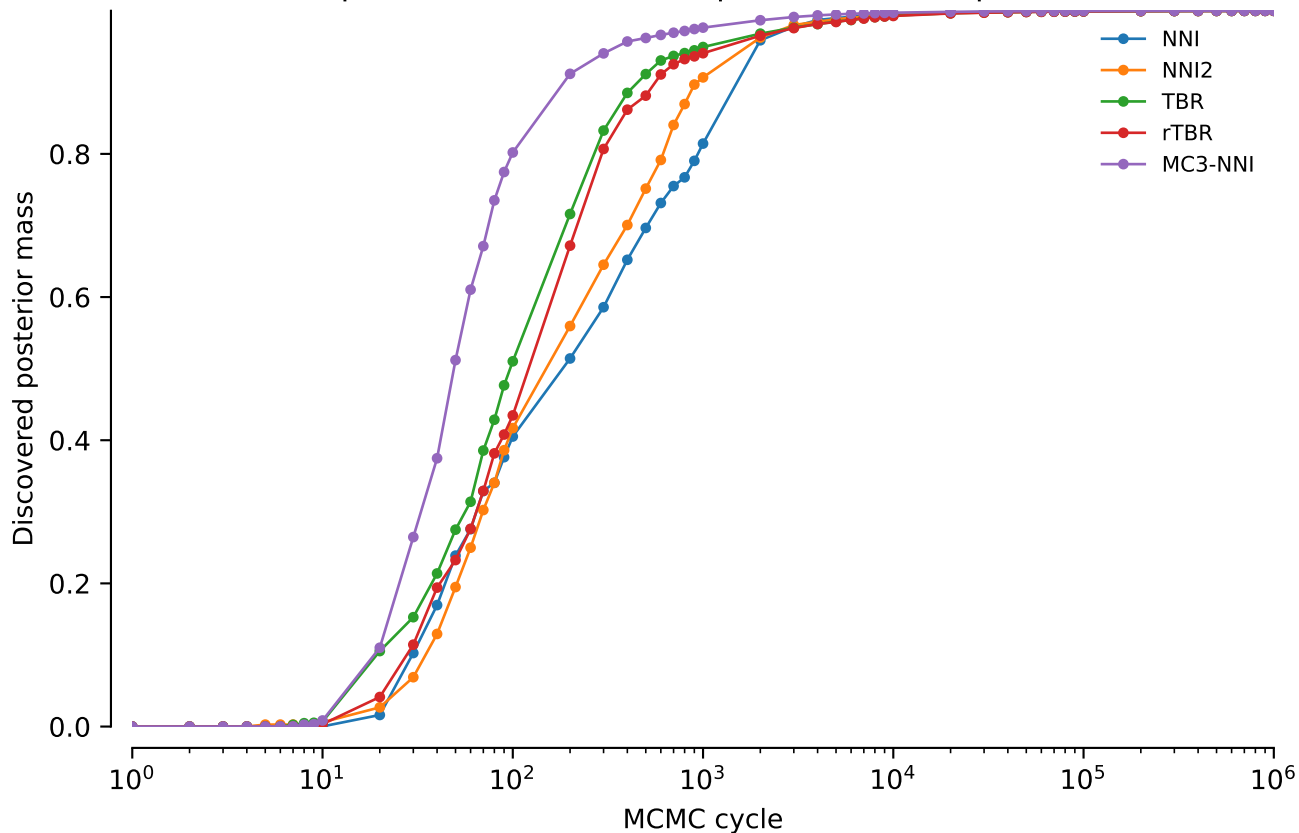
vert.atpase8.tw5: Discovered posterior mass: power = 0.1
