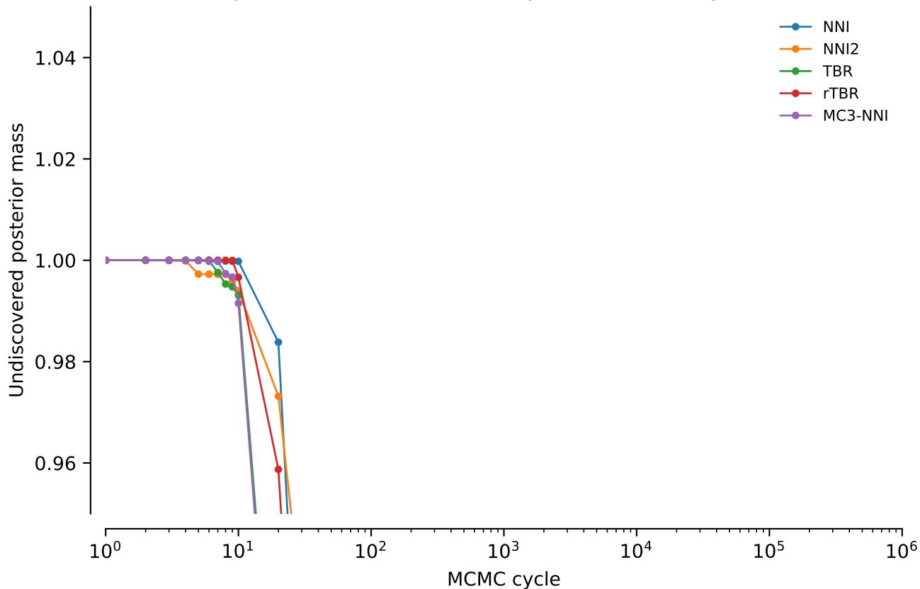
vert.atpase8.tw5: Undiscovered posterior mass: power = 0.1
