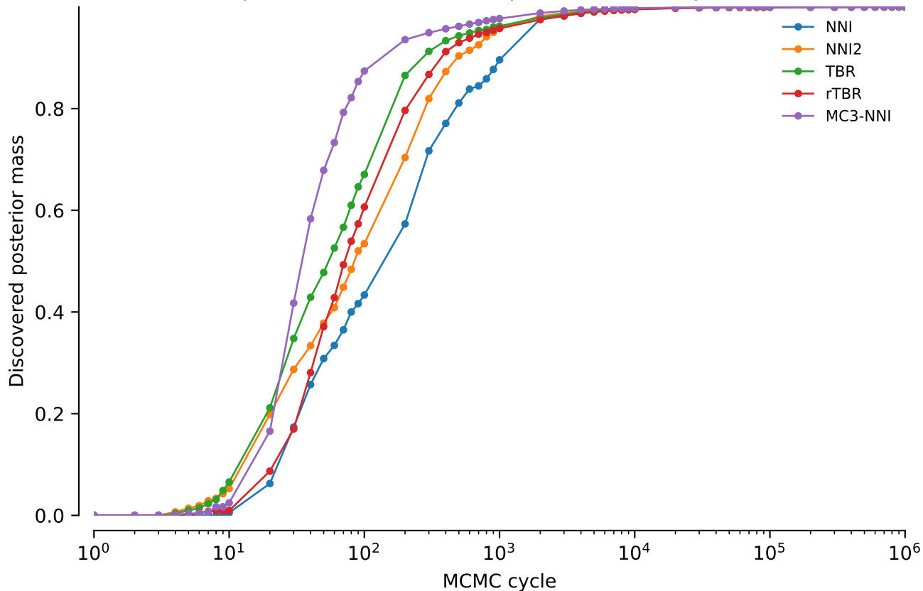
vert.atpase8.tw5: Discovered posterior mass: power = 0.2
