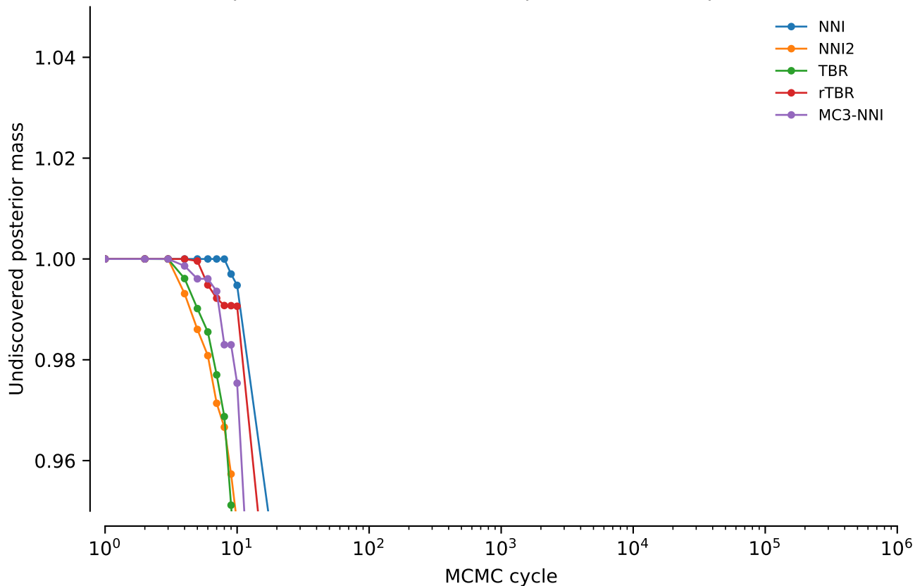
vert.atpase8.tw5: Undiscovered posterior mass: power = 0.2
