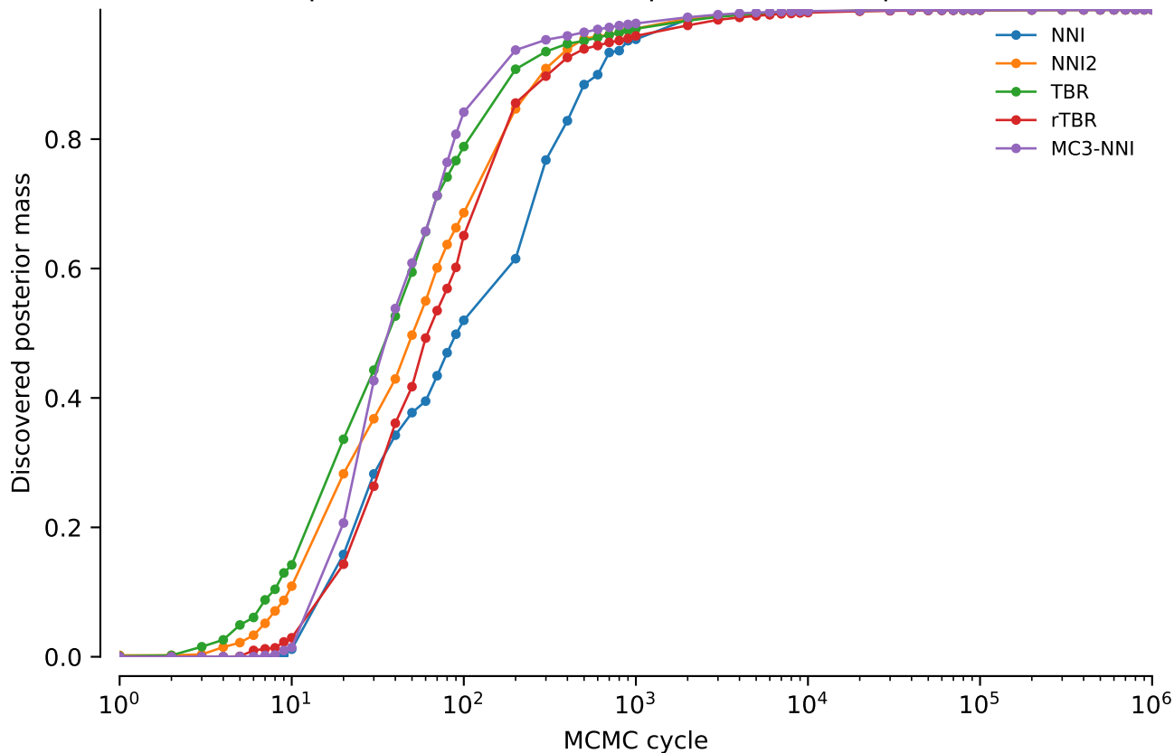
vert.atpase8.tw5: Discovered posterior mass: power = 0.3
