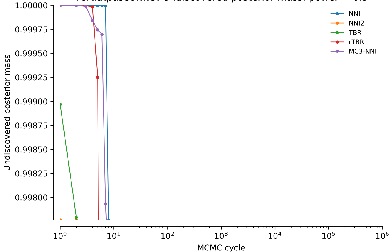
vert.atpase8.tw5: Undiscovered posterior mass: power = 0.3
