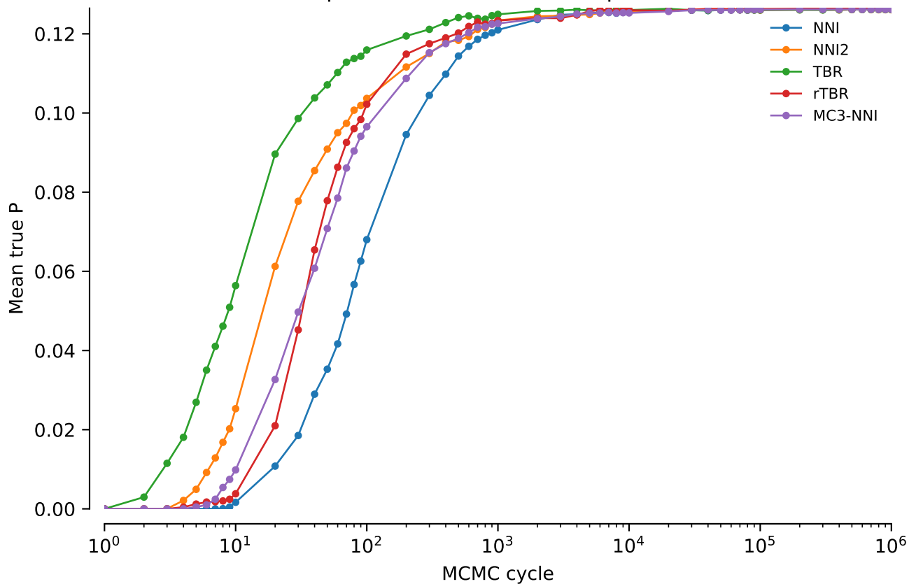
vert.atpase8.tw5: Mean true P: power = 0.4
