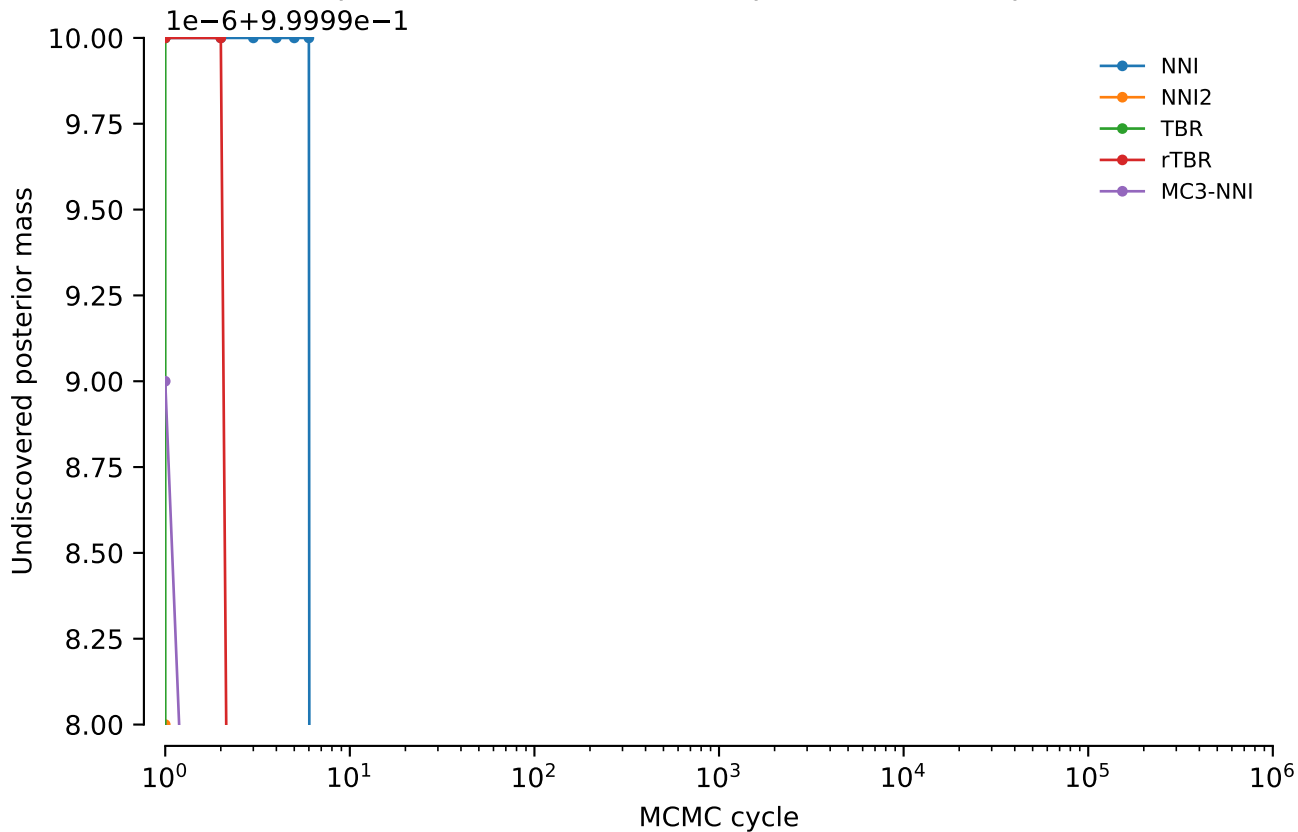
vert.atpase8.tw5: Undiscovered posterior mass: power = 0.4
