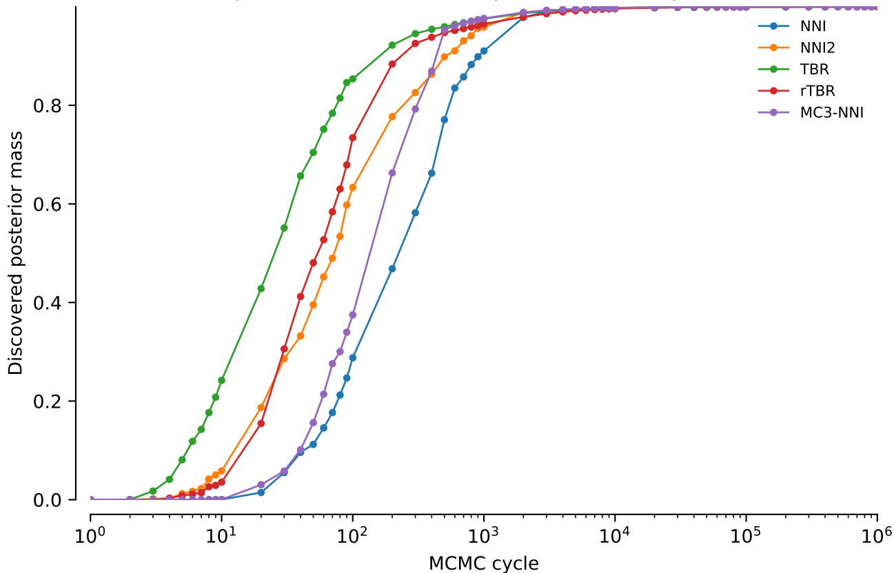
vert.atpase8.tw5: Discovered posterior mass: power = 0.5
