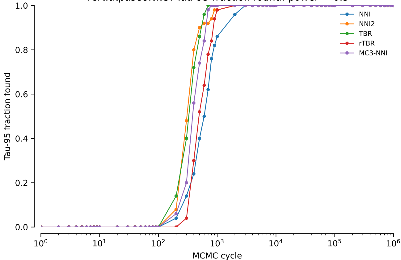
vert.atpase8.tw5: Tau-95 fraction found: power = 0.5
