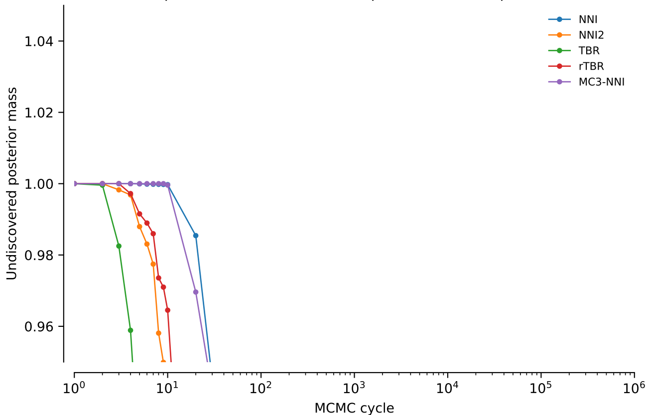
vert.atpase8.tw5: Undiscovered posterior mass: power = 0.5
