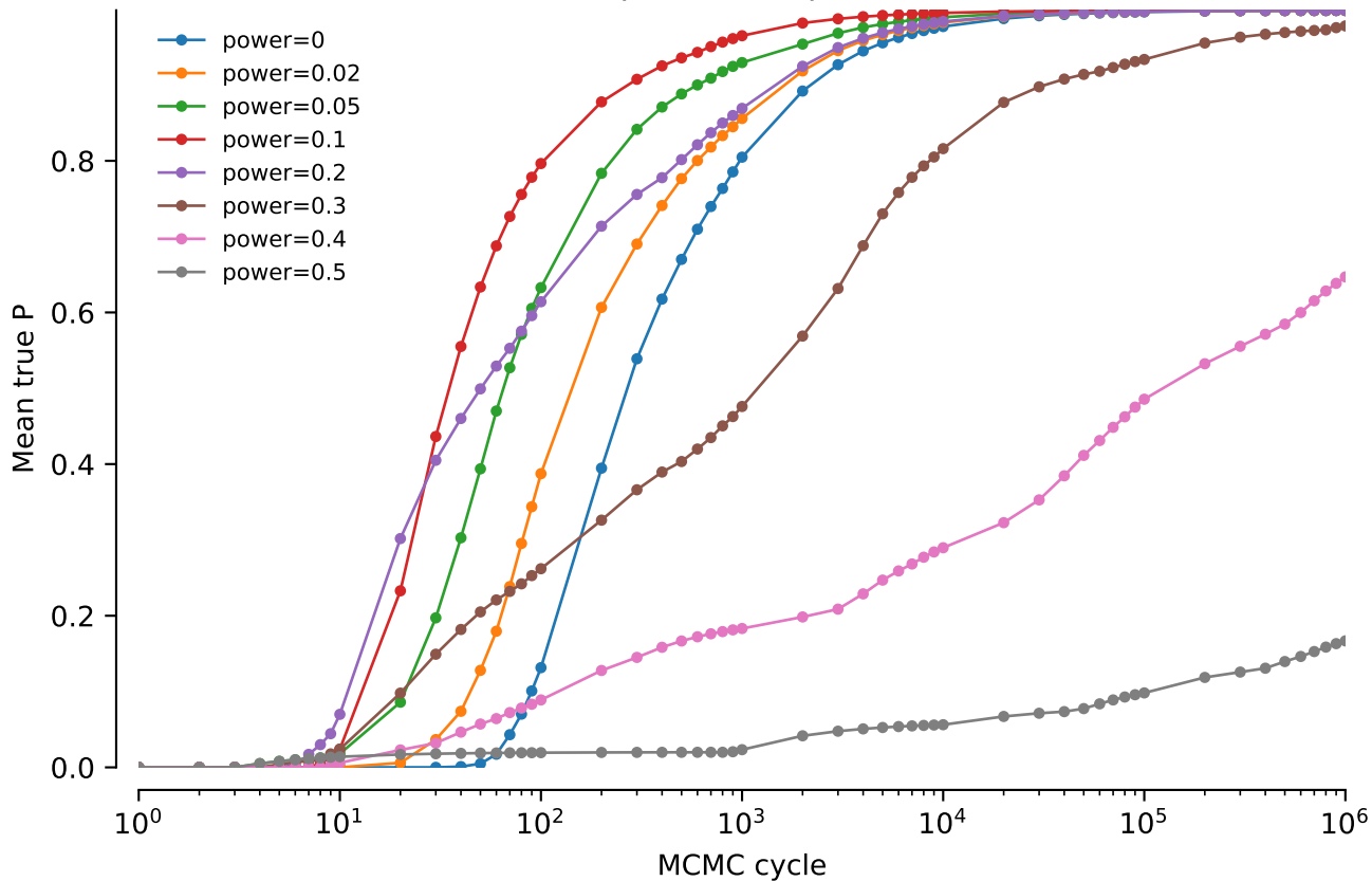
vert.coi.tw0: NNI power comparison: Mean true P
