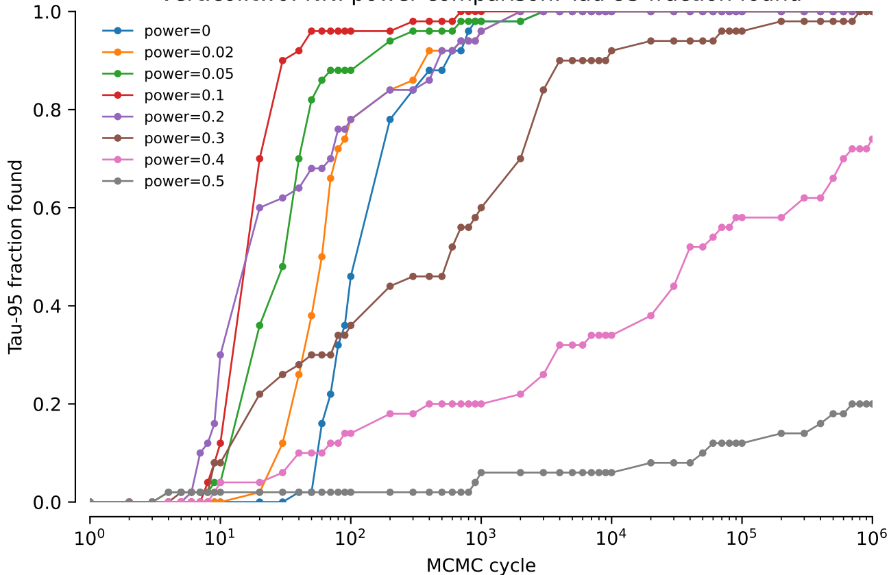
vert.coi.tw0: NNI power comparison: Tau-95 fraction found
