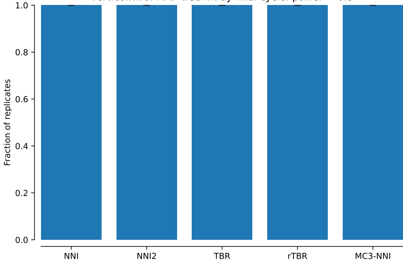
vert.coi.tw0: MAP tree hit by final cycle: power = 0.3
