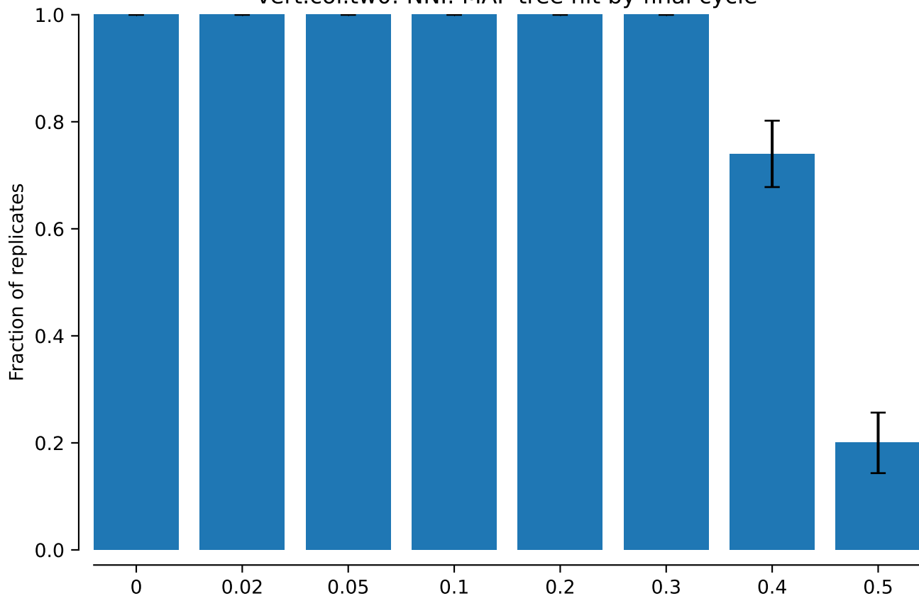
vert.coi.tw0: NNI: MAP tree hit by final cycle
