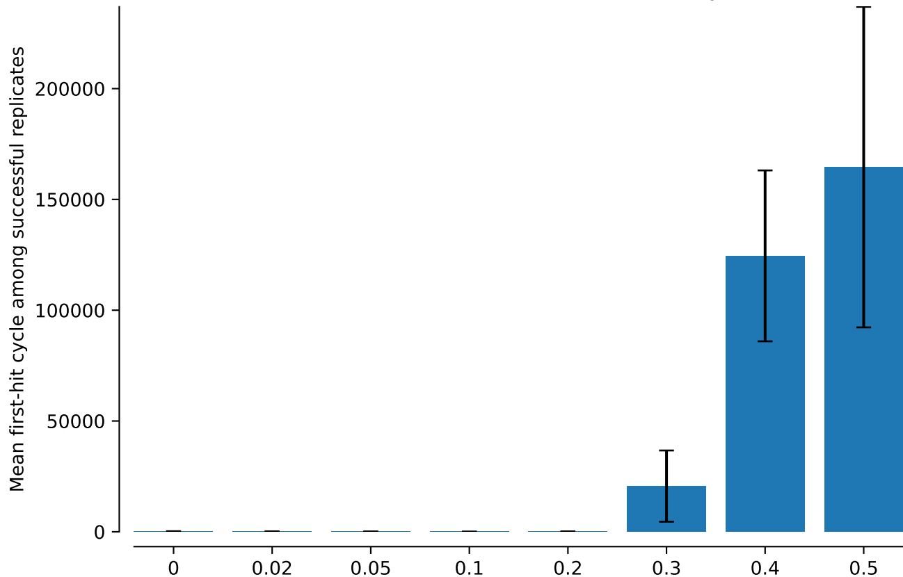
vert.coi.tw0: NNI: mean MAP first-hit cycle
