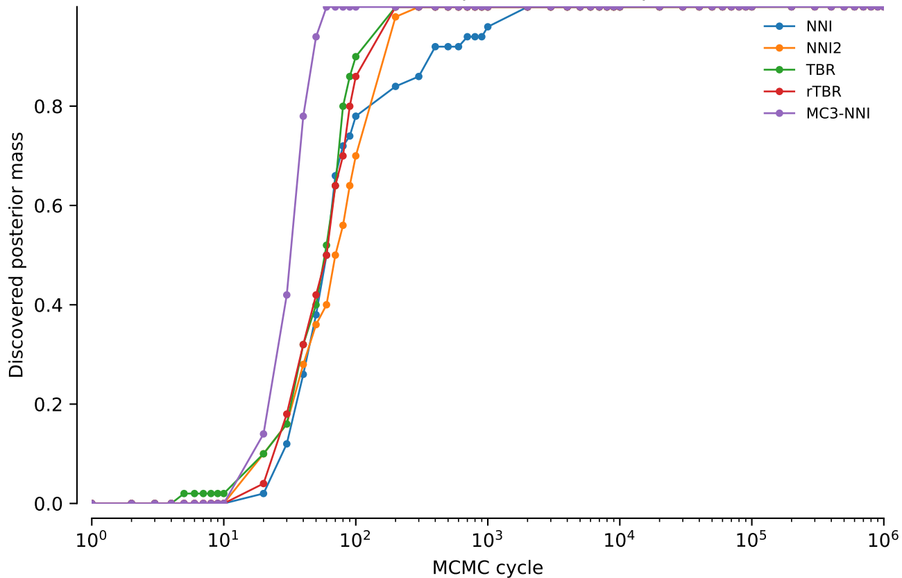
vert.coi.tw0: Discovered posterior mass: power = 0.02
