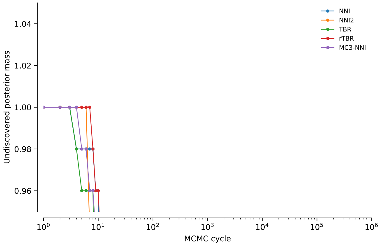
vert.coi.tw0: Undiscovered posterior mass: power = 0.05
