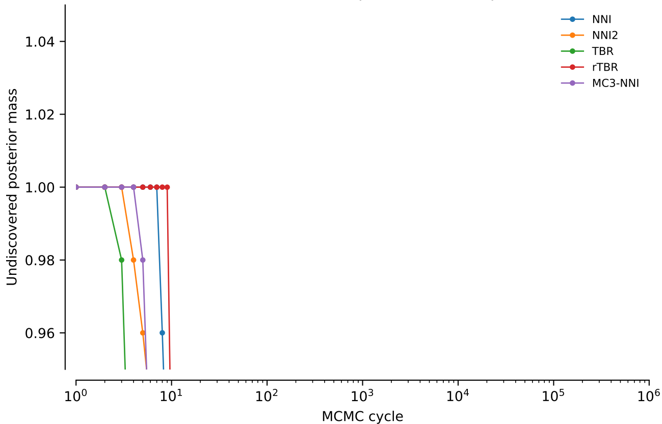
vert.coi.tw0: Undiscovered posterior mass: power = 0.1
