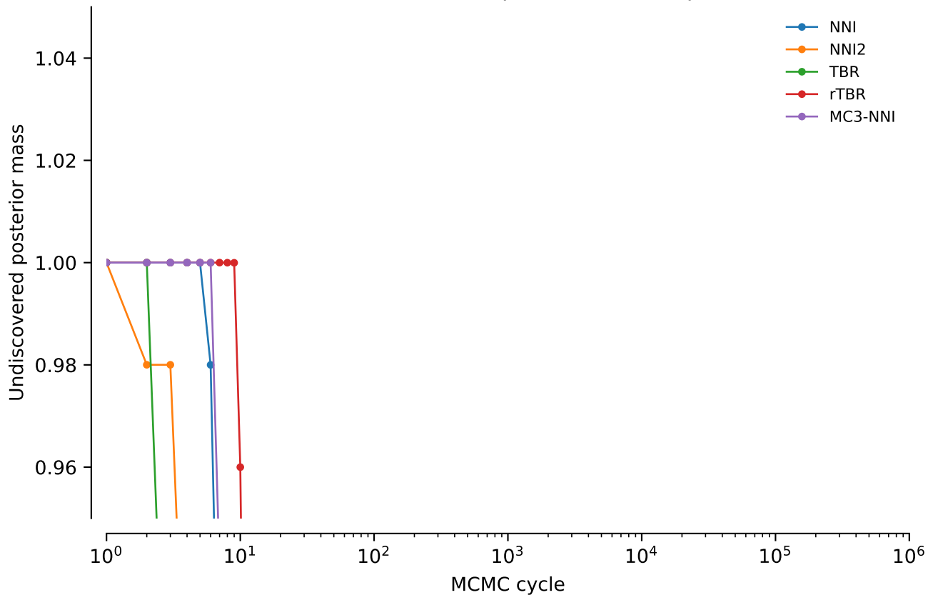
vert.coi.tw0: Undiscovered posterior mass: power = 0.2
