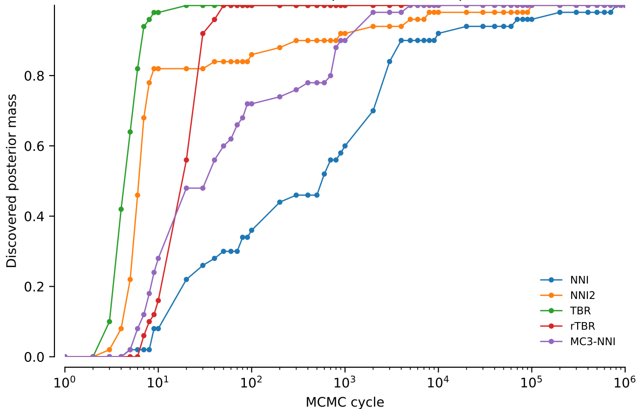
vert.coi.tw0: Discovered posterior mass: power = 0.3
