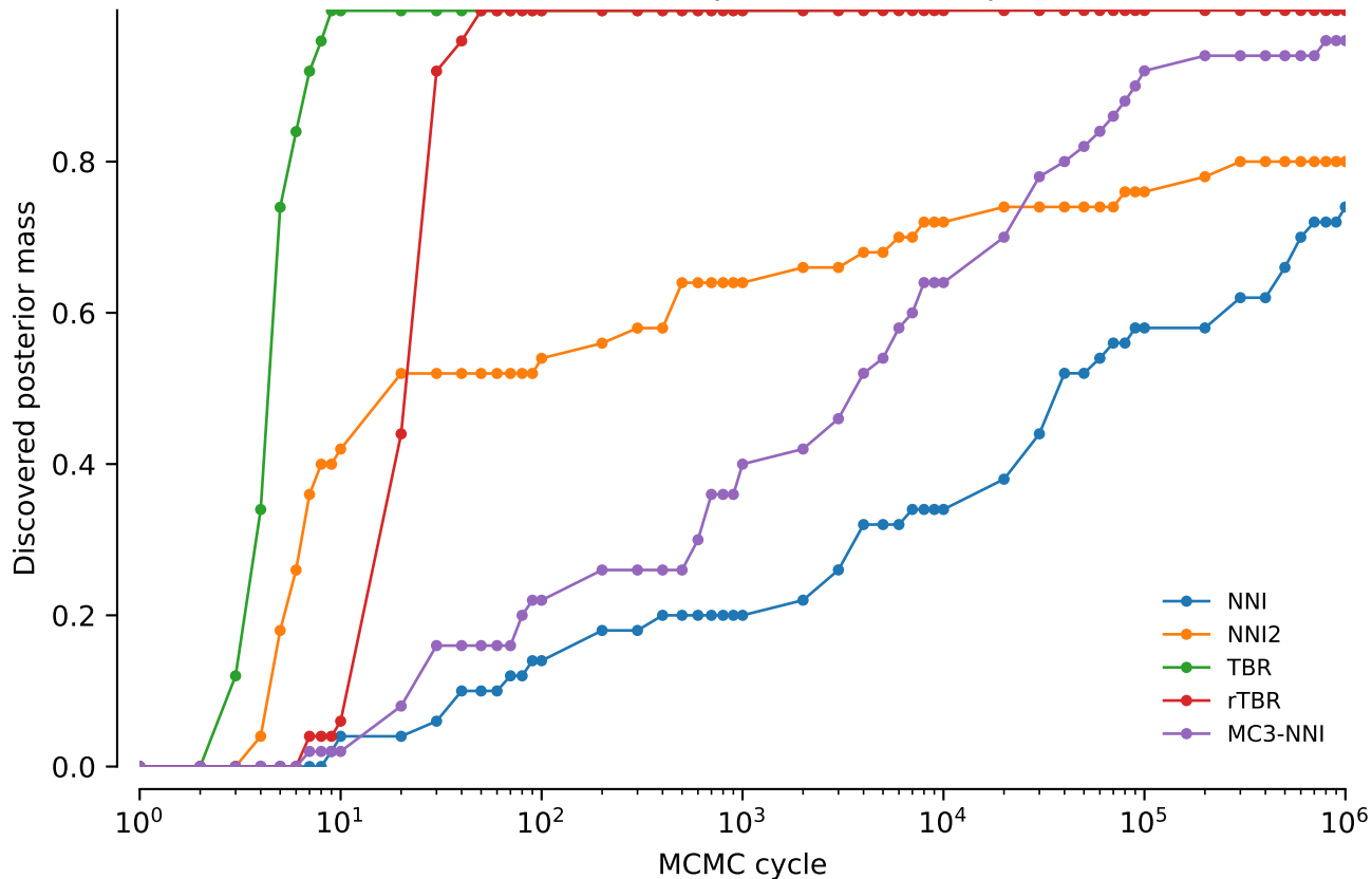
vert.coi.tw0: Discovered posterior mass: power = 0.4
