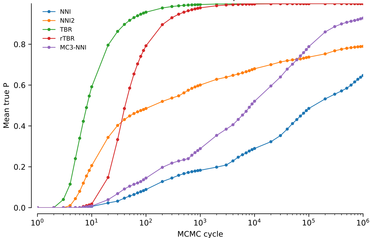
vert.coi.tw0: Mean true P: power = 0.4
