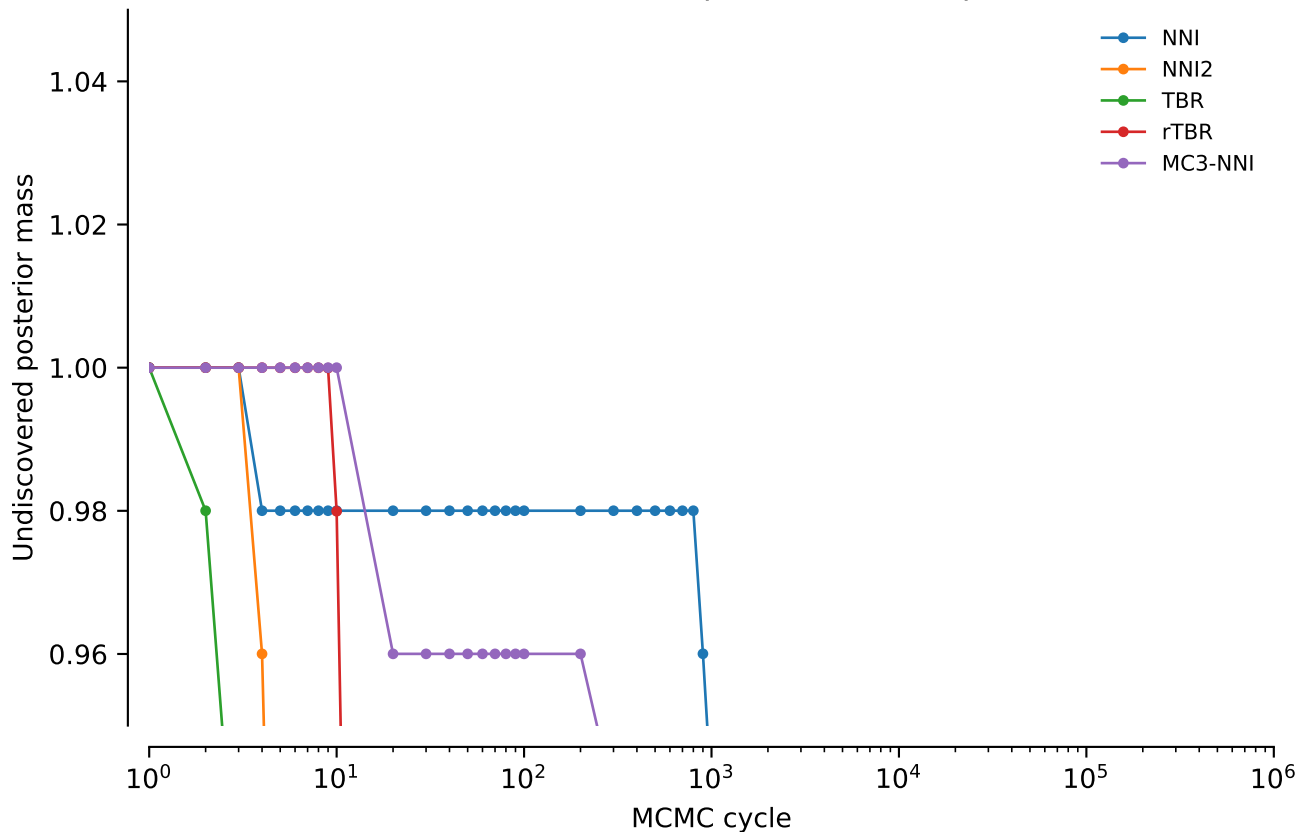
vert.coi.tw0: Undiscovered posterior mass: power = 0.5
