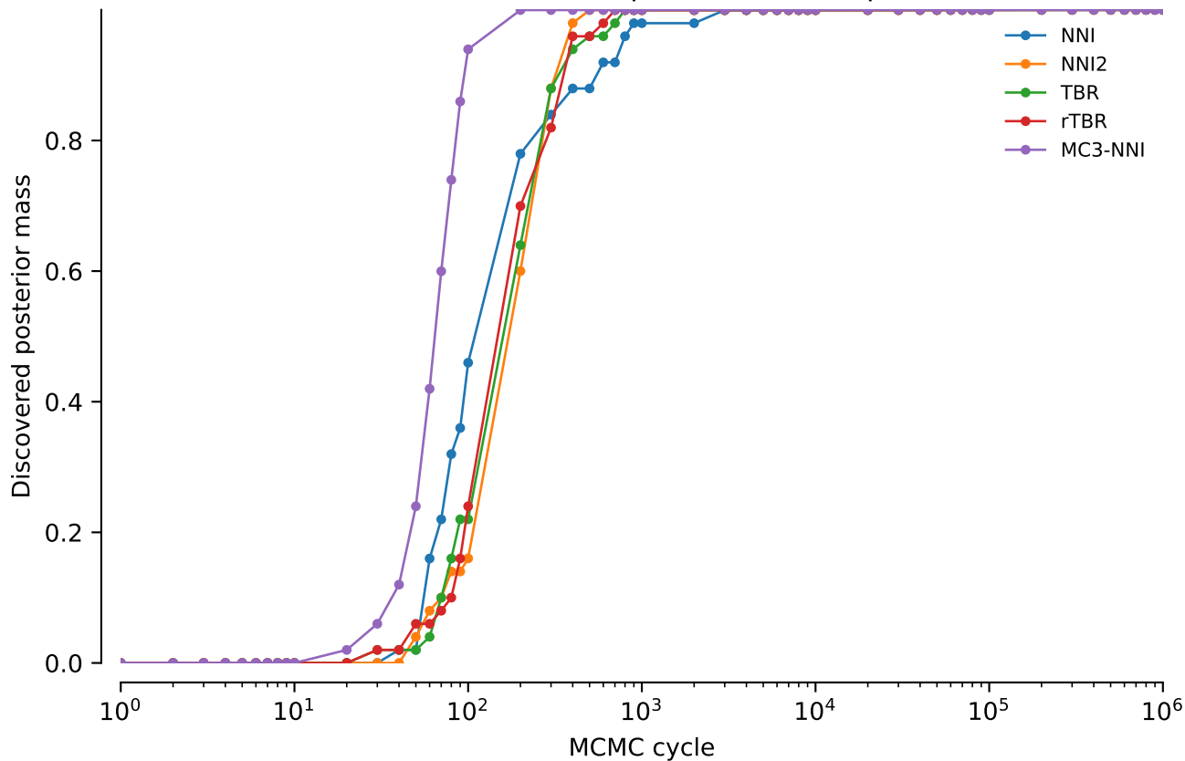
vert.coi.tw0: Discovered posterior mass: power = 0
