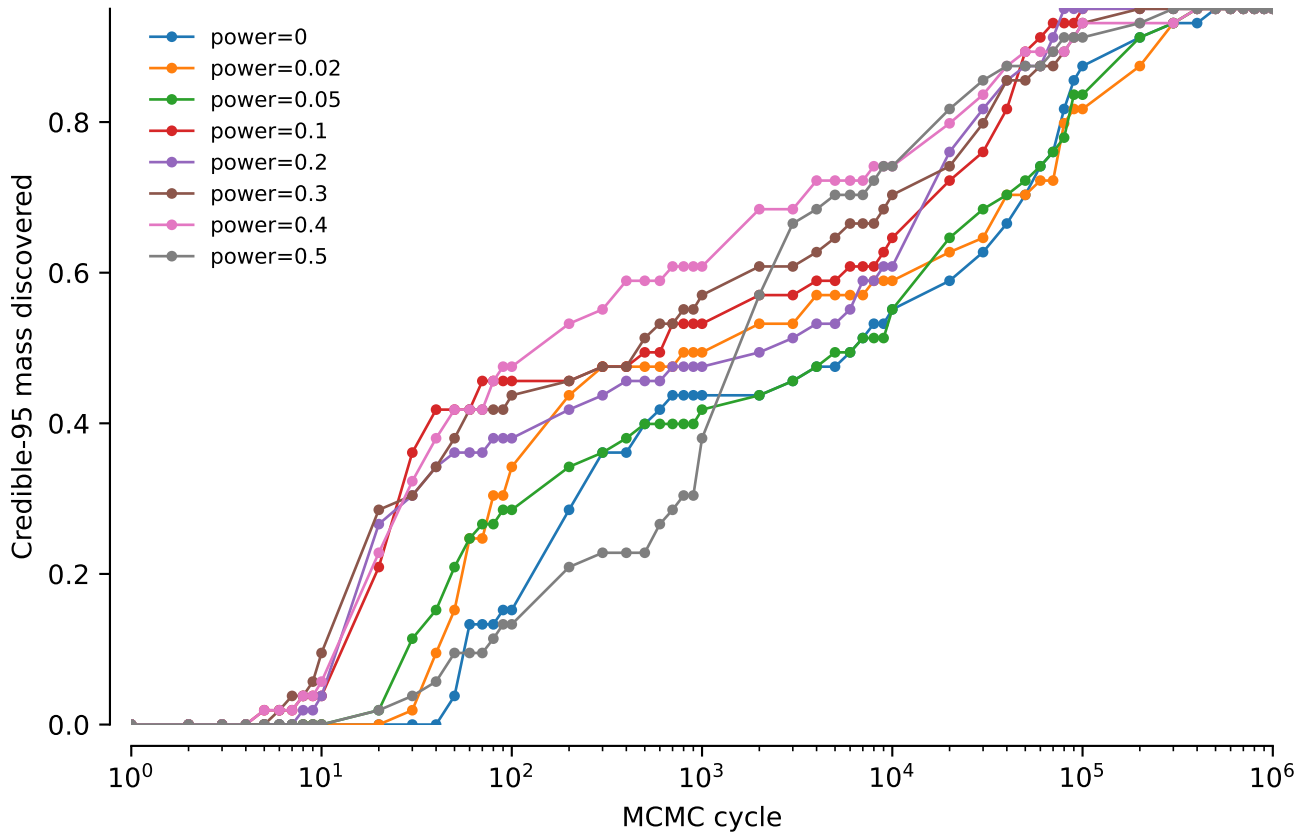
vert.coi.tw5: NNI power comparison: Credible-95 mass discovered
