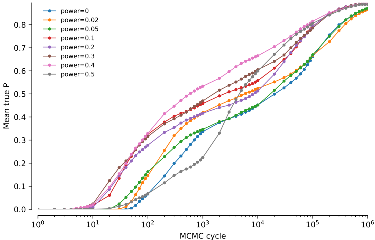
vert.coi.tw5: NNI power comparison: Mean true P
