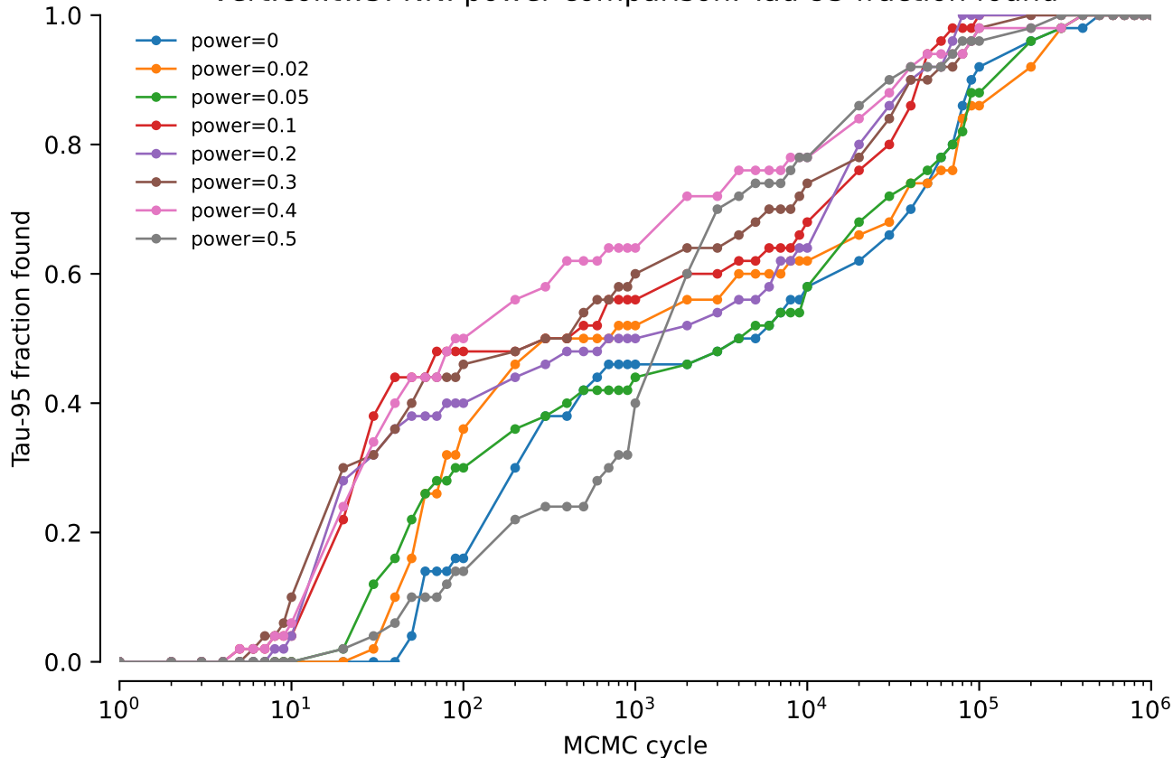
vert.coi.tw5: NNI power comparison: Tau-95 fraction found
