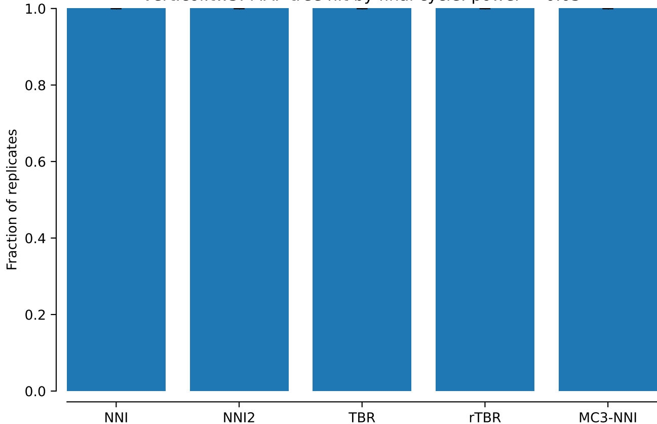
vert.coi.tw5: MAP tree hit by final cycle: power = 0.05
