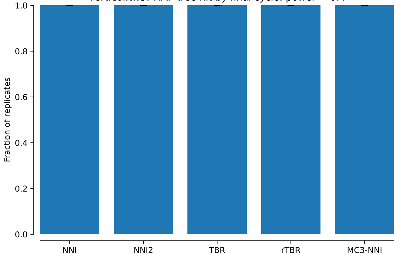
vert.coi.tw5: MAP tree hit by final cycle: power = 0.4
