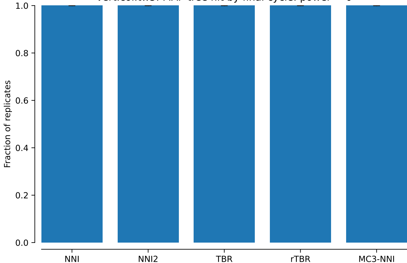
vert.coi.tw5: MAP tree hit by final cycle: power = 0
