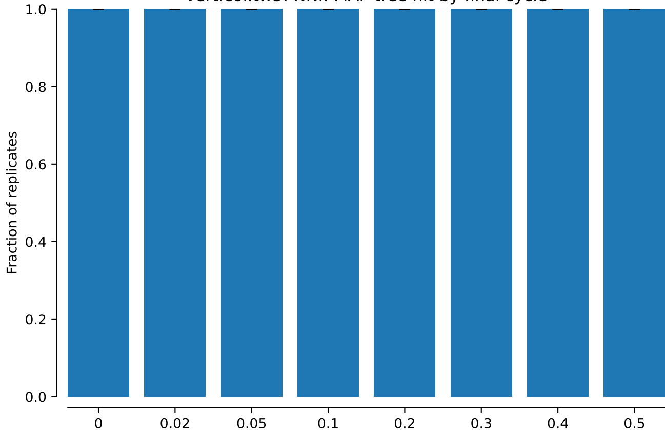
vert.coi.tw5: NNI: MAP tree hit by final cycle
