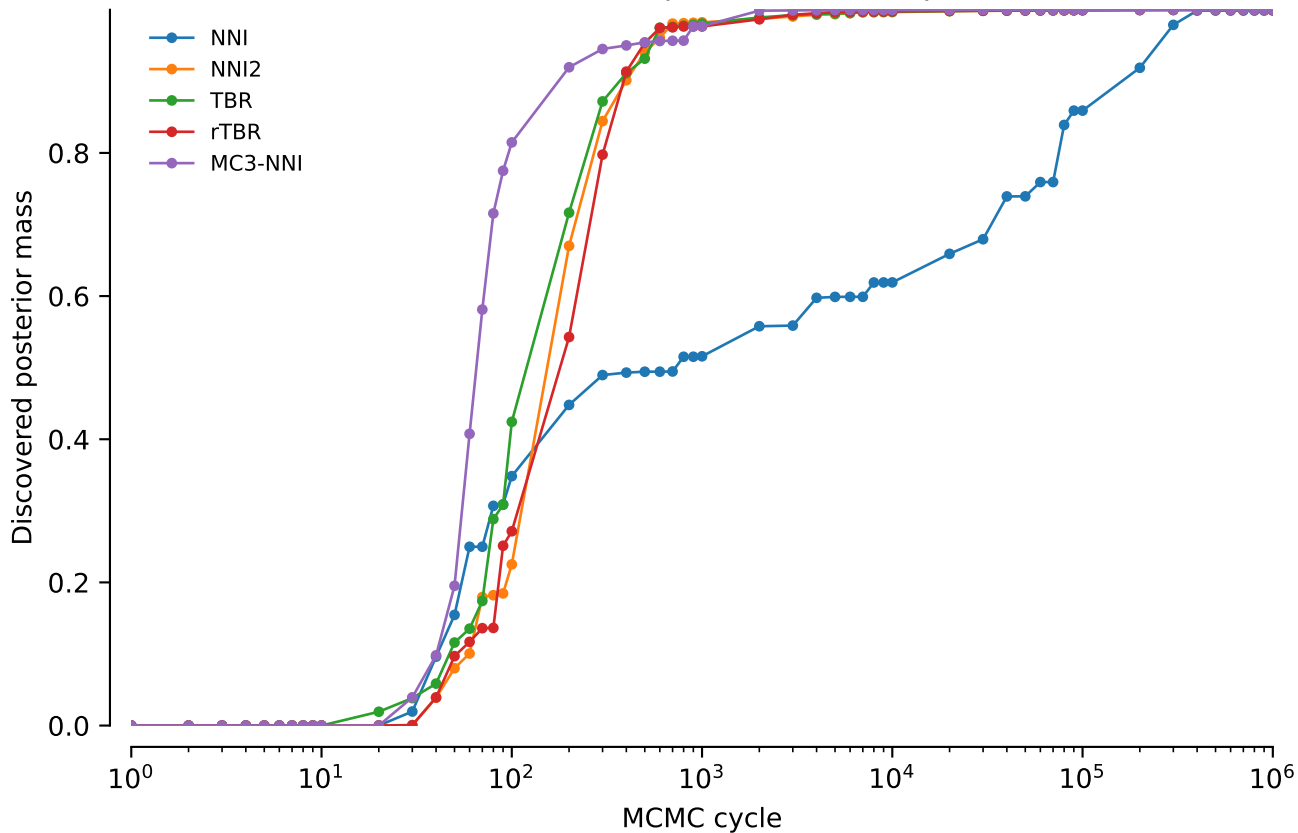
vert.coi.tw5: Discovered posterior mass: power = 0.02
