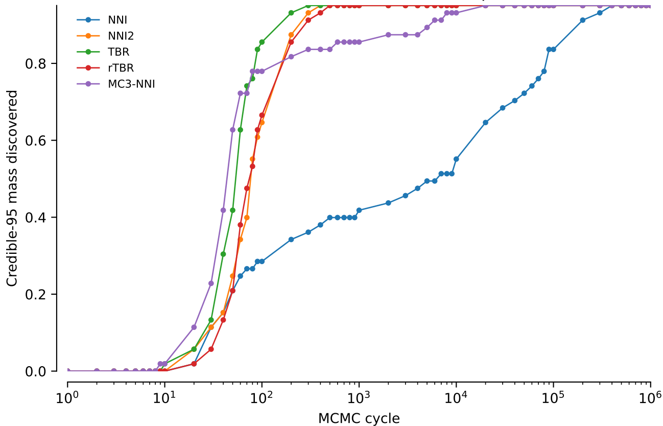
vert.coi.tw5: Credible-95 mass discovered: power = 0.05
