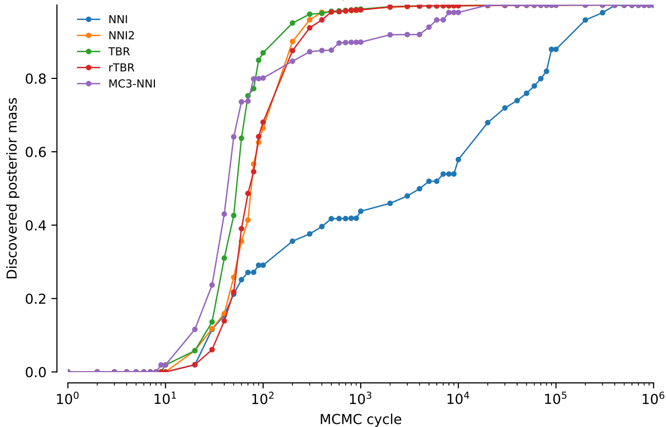
vert.coi.tw5: Discovered posterior mass: power = 0.05
