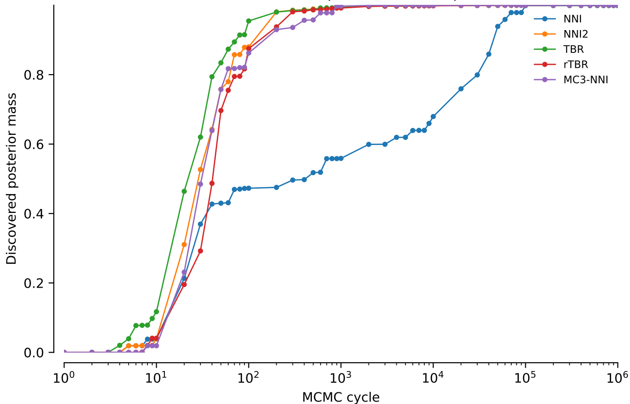
vert.coi.tw5: Discovered posterior mass: power = 0.1
