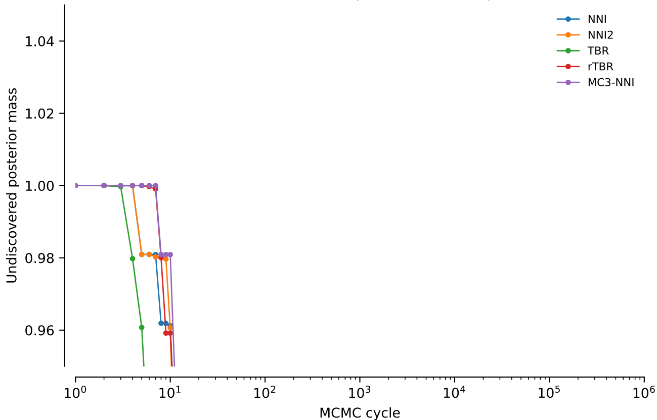
vert.coi.tw5: Undiscovered posterior mass: power = 0.1
