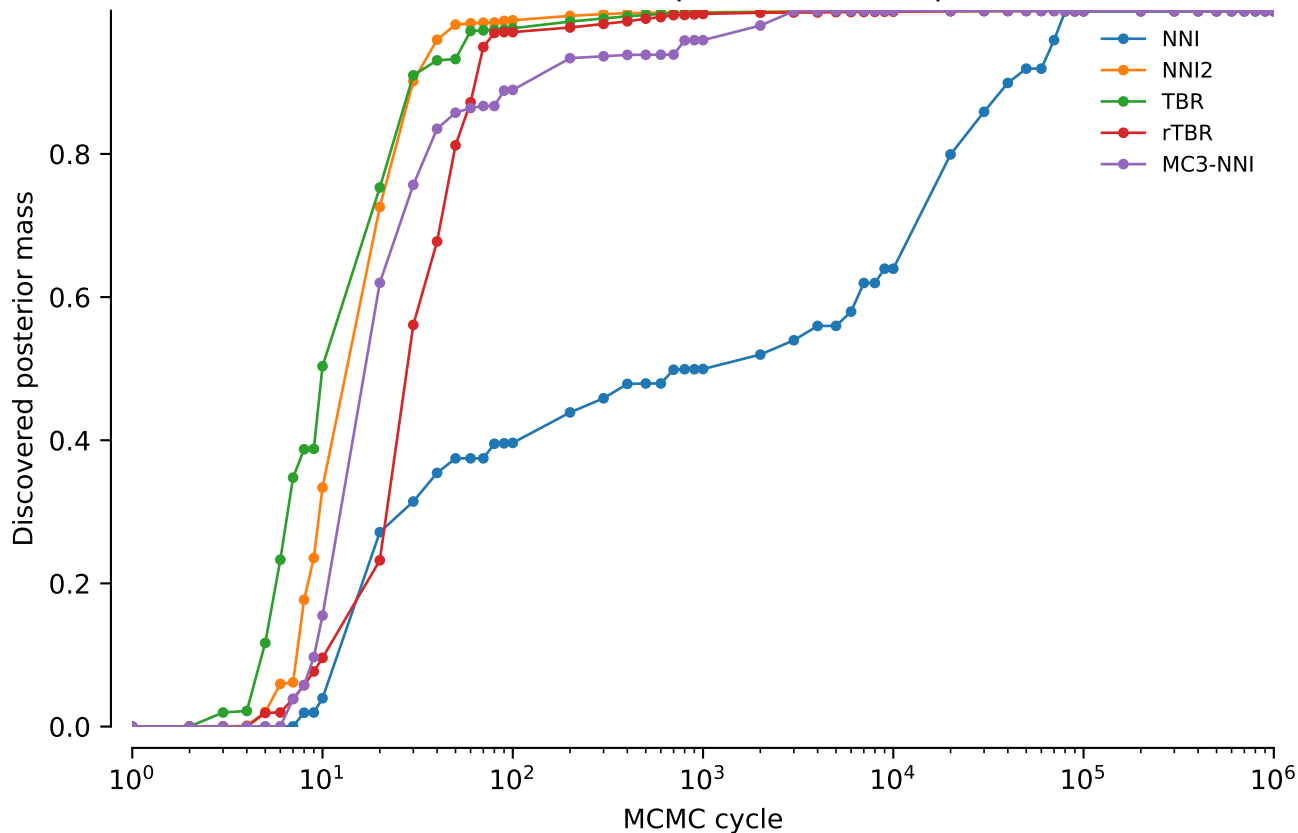
vert.coi.tw5: Discovered posterior mass: power = 0.2
